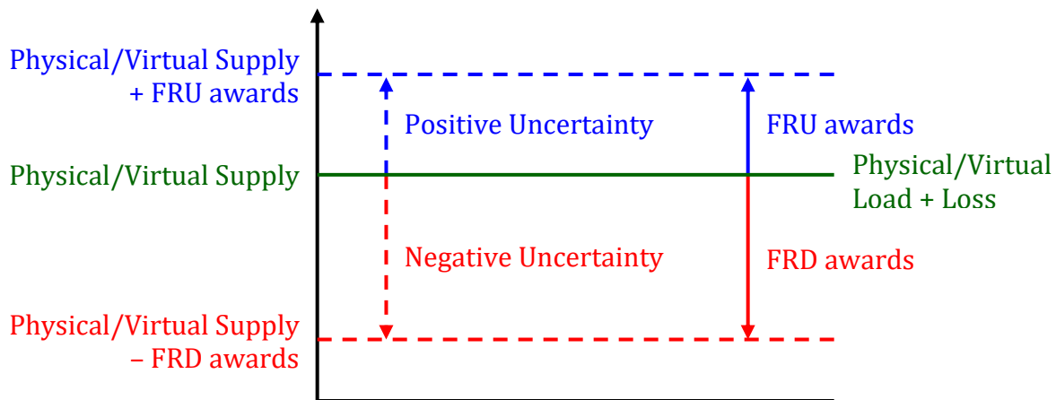
Figure 1. Energy and Flexible Ramp Up/Down targets
