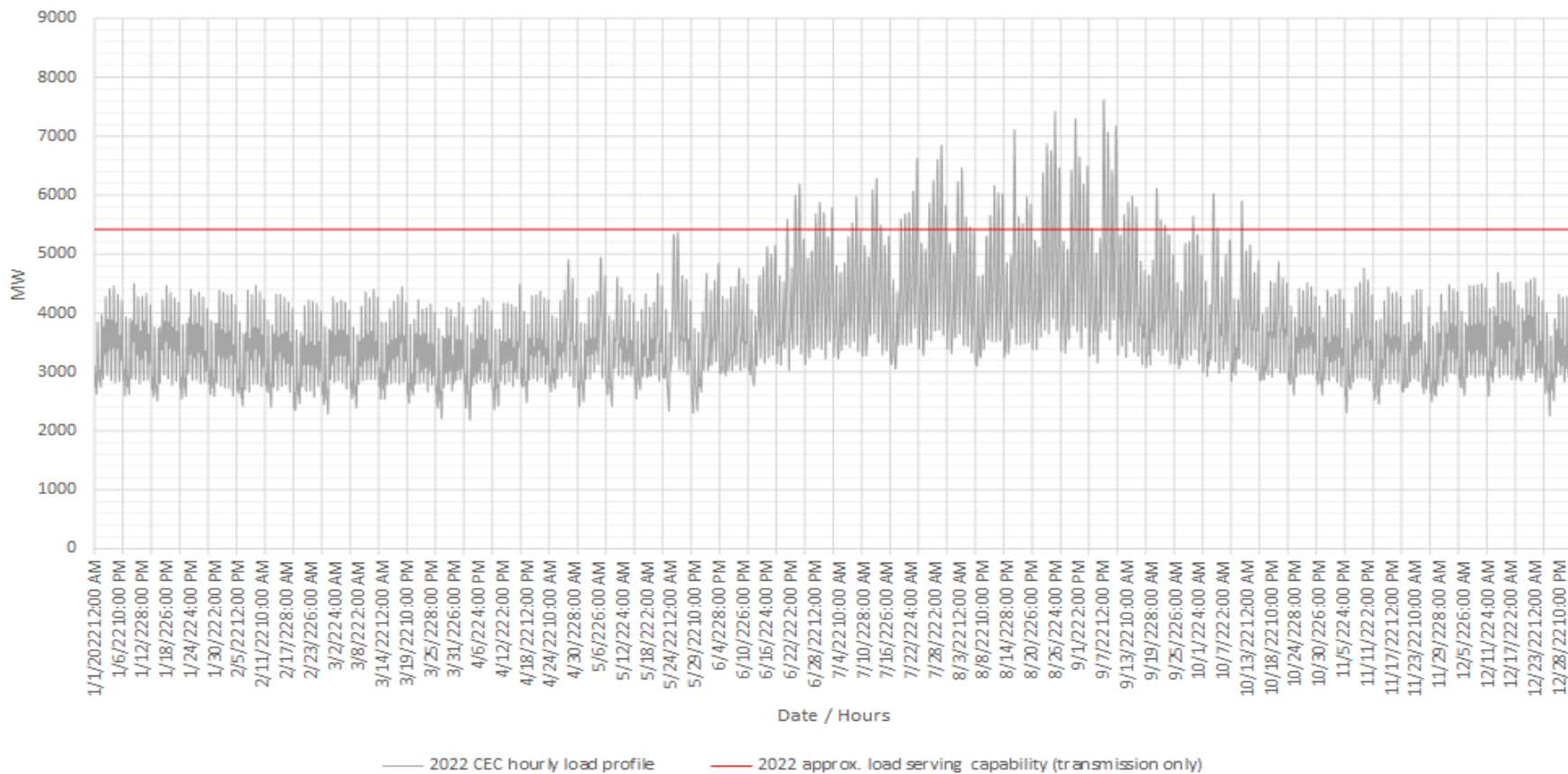
Eastern LA Basin Sub-area: 2022 CEC hourly load profile & approx. load serving capability (transmission only)
