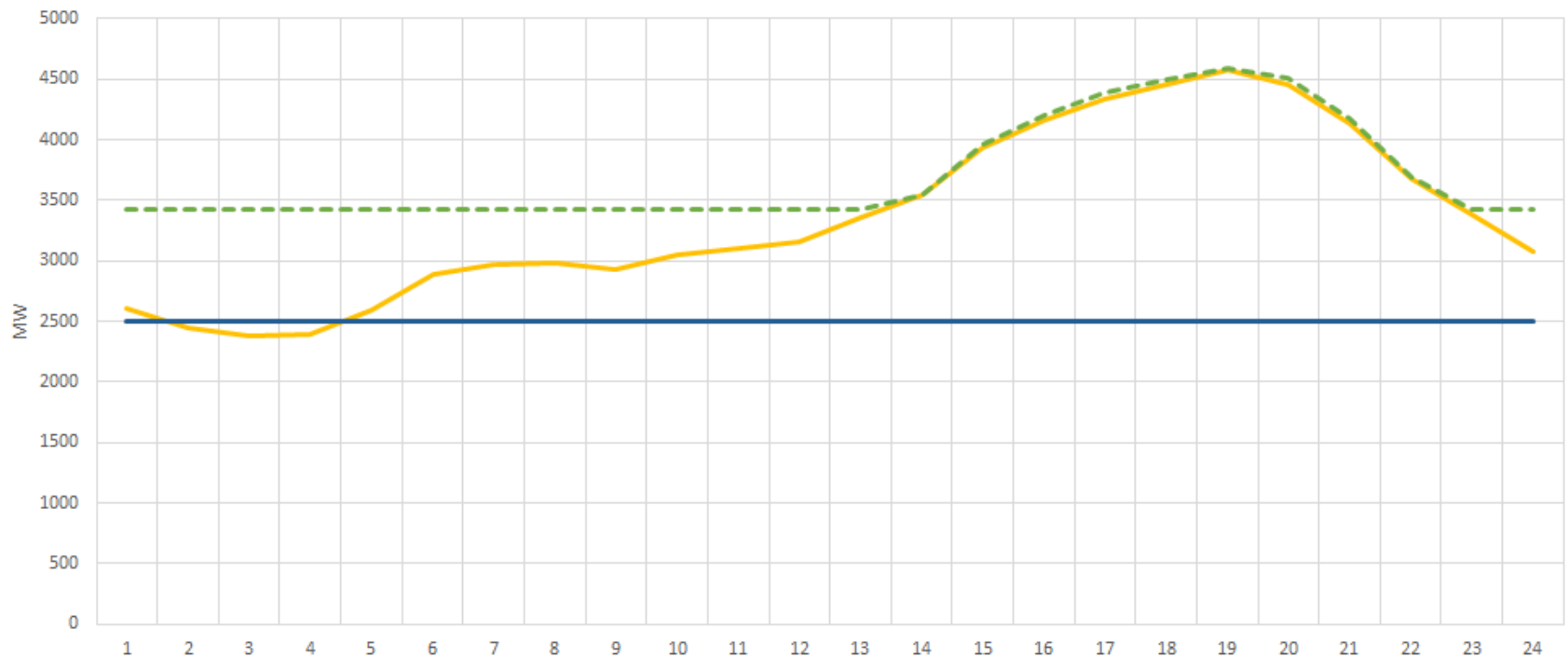
San Diego-Imperial Valley Area: 2022 peak day load profile & approx. LSC (transmission + LCR Gen + ES) Approx. amount of storage that can be added to this area from charging restriction perspective = 1165 MW and 6690 MWh. Approx. max 4-hr storage = 670
